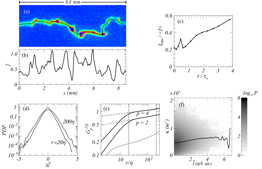
FIG. 8. (a) Image of a line of NO molecules for delay time t = 30 \mu\text{s} ( 2.3 \tau_\eta ). The black line traces its backbone \mathbf{x}(s) . (b) Normalized line intensity \tilde{I}(s) as a function of the curvilinear coordinate s along the line (the length of this line is larger than the 6.4 mm width of the image). The intensity \tilde{I}(s) has been filtered using a binomial filter with width 2\eta . (c) Rms intensity fluctuation along lines as a function of delay time between writing and reading. (d) PDF of increment \delta \tilde{I}(r) for separations r = 20\eta and 200\eta and delay time t = 50 \mu\text{s} ( 3.8 \tau_\eta ). (e) Structure functions G_p^{1/p}(r) = \langle (\tilde{I}_i(s+r) - \tilde{I}_i(s))^p \rangle_{i,s}^{1/p} for orders p = 2, 4 and delay time t = 50 \mu\text{s} . Dashed lines: fits of inertial range behavior G_p(r) \sim r^{\zeta_p} , with \zeta_p \approx 0.1 p . Gray line: G_2^{1/2} of lines at t = 2 \mu\text{s} , which provides an estimate of the uncertainty of the results at t = 50 \mu\text{s} . (f) Joint histogram P(\kappa, I) of curvature \kappa and intensity I , line: mean \langle \kappa \rangle as a function of intensity I . Curvatures were computed over intervals l_c = 15\eta . The shades of gray are on a logarithmic scale. The correction for the intensity variation of writing and reading lasers over the image plane was discussed in Sec. III B.
